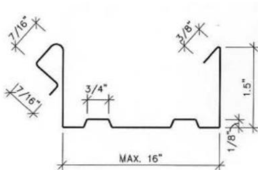
1.5" Snap Lock Panel Dimensions
